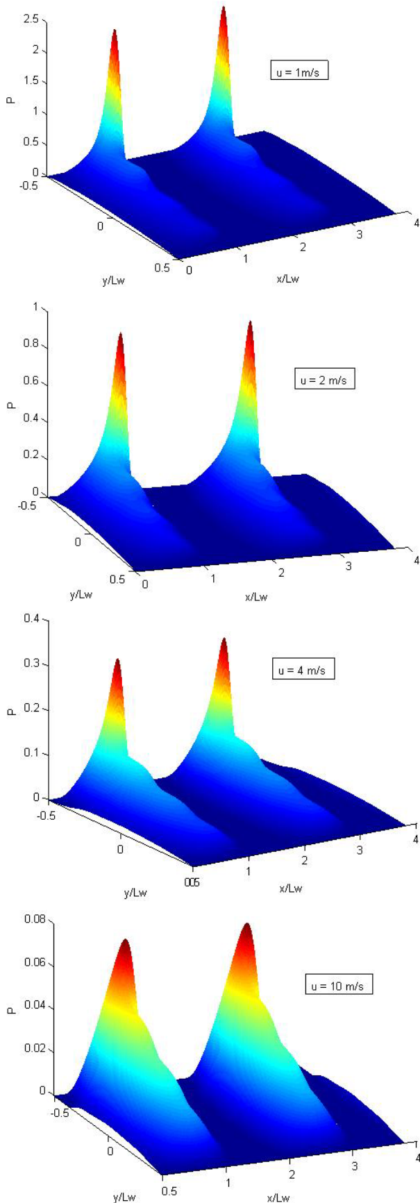
Figure 7. Pressure distribution as a function of rotational speed
