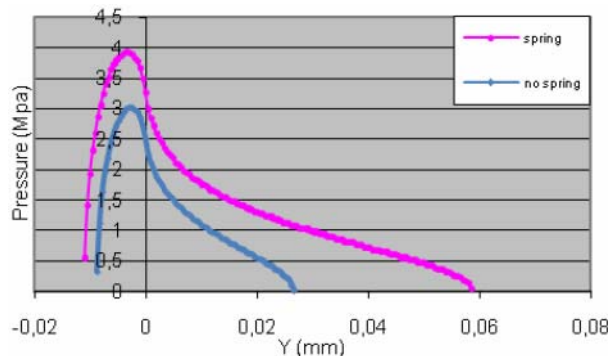
Figure 4. Pressure distribution with and without the Garter spring
