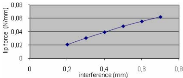
Figure 3. Lip force variation with interference
