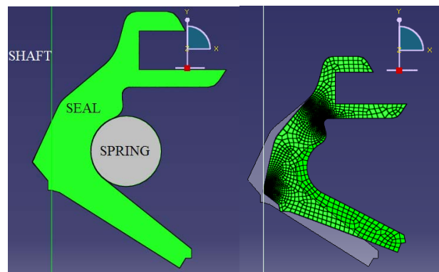
Figure 1. Seal design and mesh
