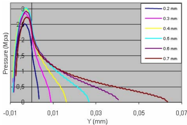
Figure 2. Pressure distribution for different shaft interference
