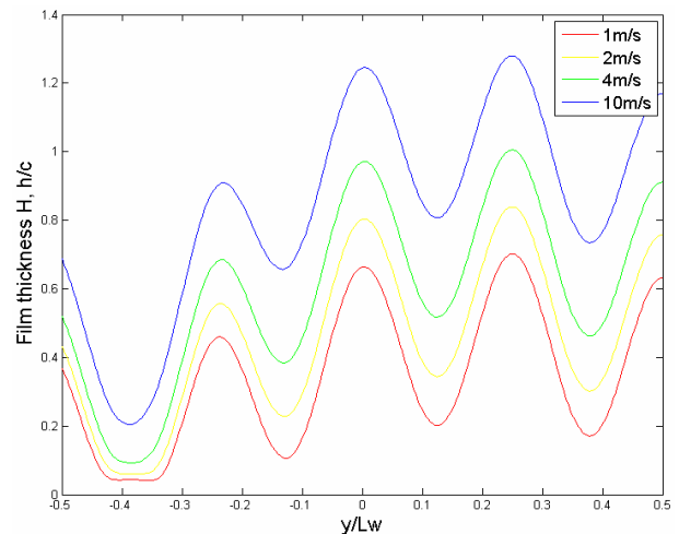
Figure 8. Film thickness as a function of the shaft rotational speed
