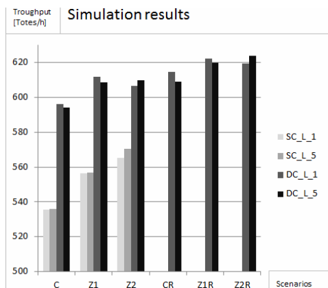
Figure 13. Simulation results, class-based storage and sequencing of retrieval requests, Acceleration and Velocity elevator = 7 m/s 2
