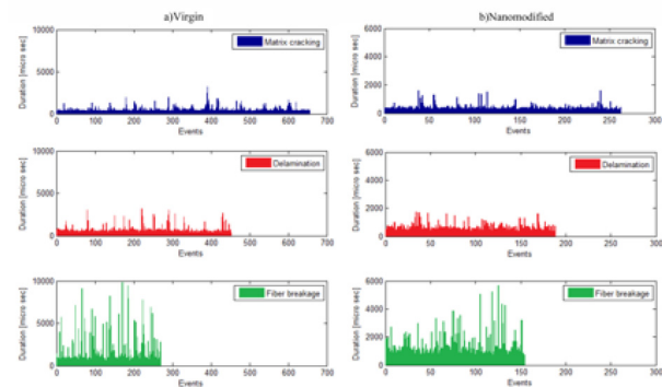
Figure 3: Duration vs. number of counts (a) virgin and (b) nanommodified
