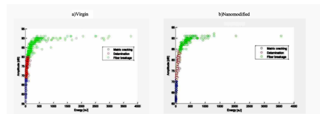
Figure 4: Amplitude vs. Energy of: (a) virgin and (b) Nanommodified
