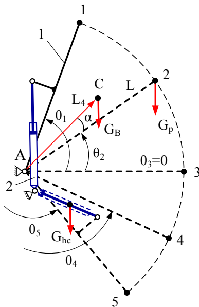
Figure 1. Graphical layout of the boom specific positions
